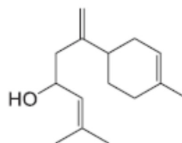
\beta - Atlantol
