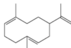
Germacrene A
